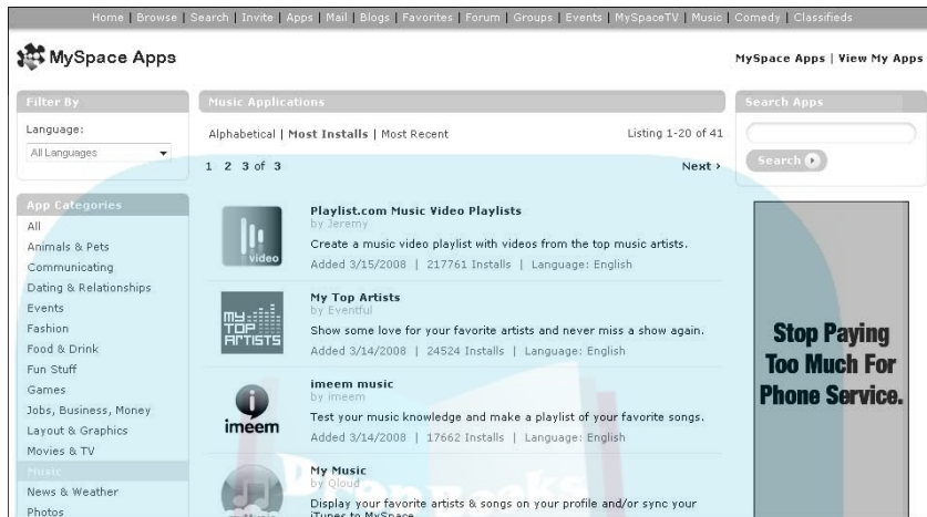
Figure 12-12: Music applications.
